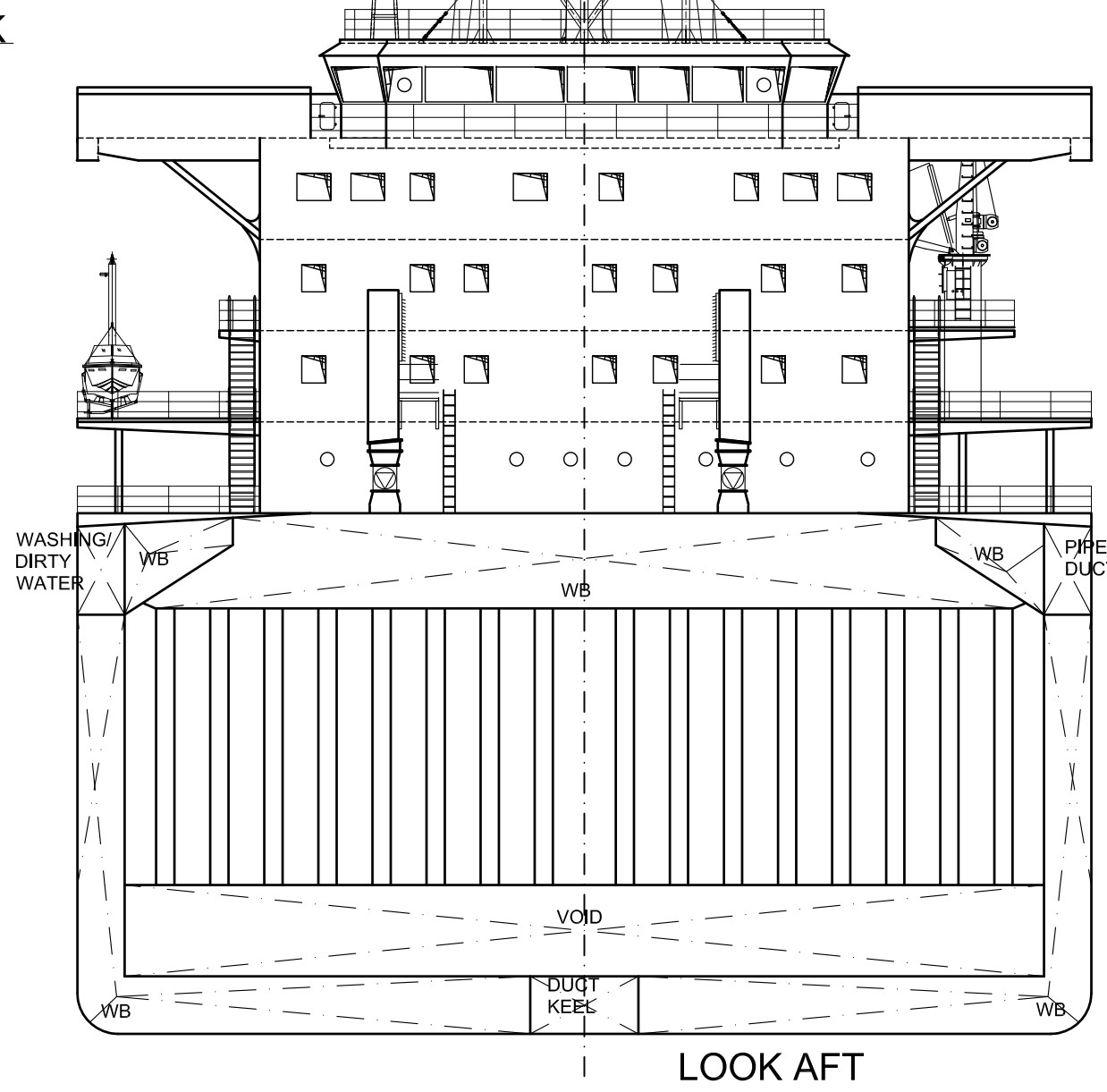
COMP. BRIDGE DECK 29.30 m ab. BL
